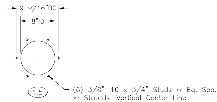
Negative Air Flange Detail
